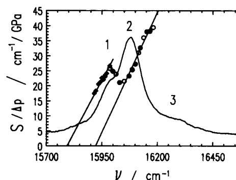
FIGURE 5 Frequency shift per unit pressure as a function of burn frequency. The straight lines represent least square fits to the data in the pure band regions. Their extrapolations to zero determine the vacuum frequencies \nu_{\text{vac},1} and \nu_{\text{vac},2} of the dye species. Their slope is twice the compressibility. The experiment was repeated three times. The corresponding data are represented with different symbols.
